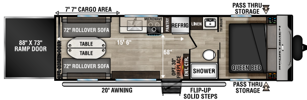
270THSE - TOY HAULER UYW - 5,400 | Exterior Length - 30'10" | Sleeps - 6
