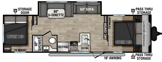
301DBSE UYW - 6,180 | Exterior Length - 32'10" | Sleeps - 8
