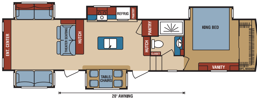
G381REF UVW 12,120 • Dry Hitch Wt. 2,250 • NCC 2,875 • GVWR 14,995 • Length 40' 6"
